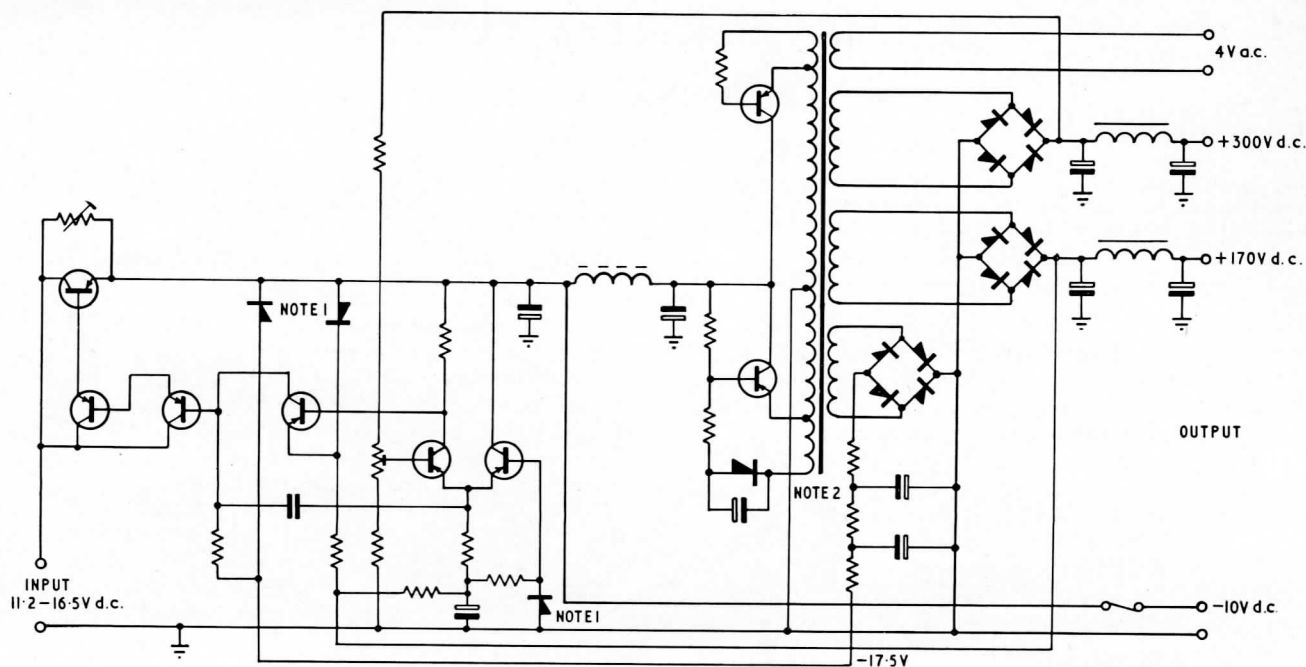
Notes: 1. Zener diodes. 2. Saturated low-hysteresis transformer.
